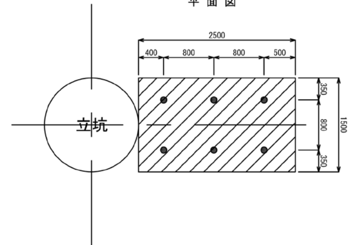
③注入範囲 幅1.5m×長さ2.5m
