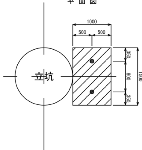
①注入範囲 幅1.5m×長さ1.0m
