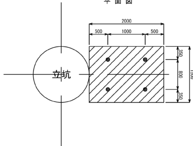
②注入範囲 幅1.5m×長さ2.0m
